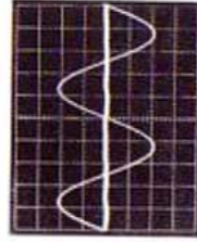
New Class A amplifier output waveform and distortion waveform (at 20 kHz)
